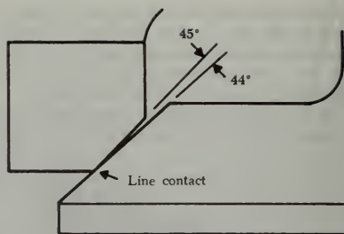
FIGURE 10-14. Interference fit of valve and valve seat.
